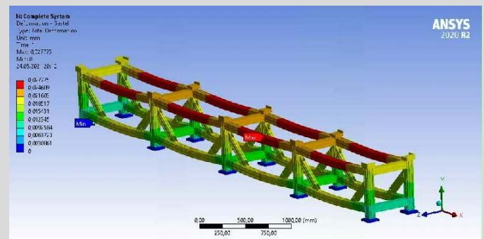
FE-Simulation Maschinengestell
